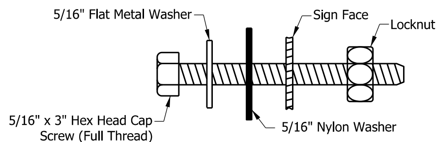
SIGN BOLT DETAIL
