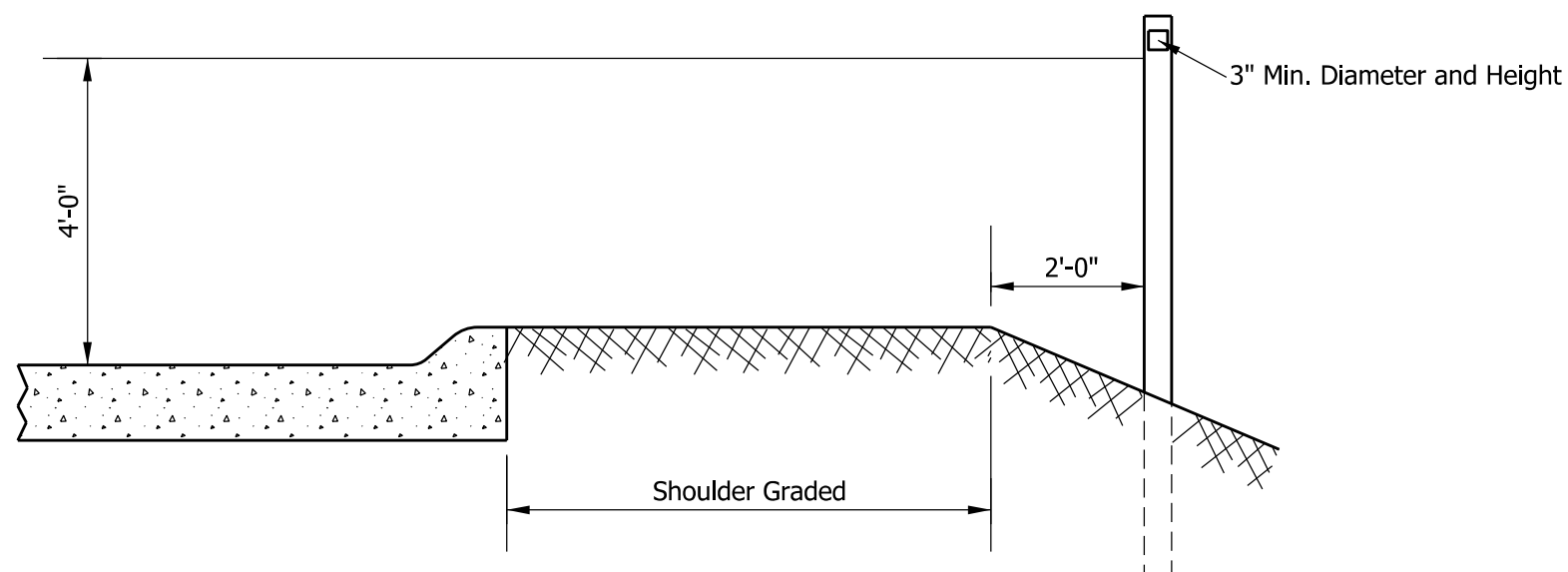
SLOPING CURB SECTION
