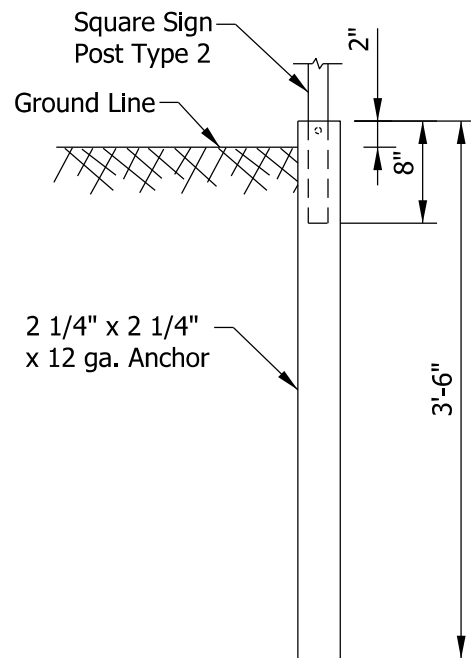
UNREINFORCED ANCHOR BASE
