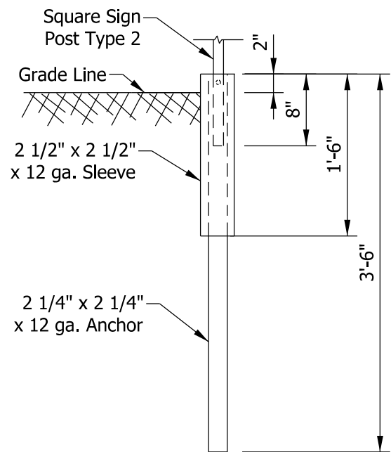
REINFORCED ANCHOR BASE
