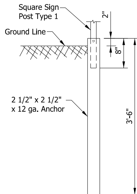
UNREINFORCED ANCHOR BASE
