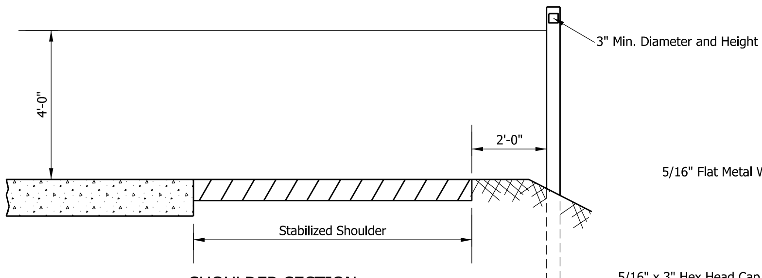
SHOULDER SECTION
