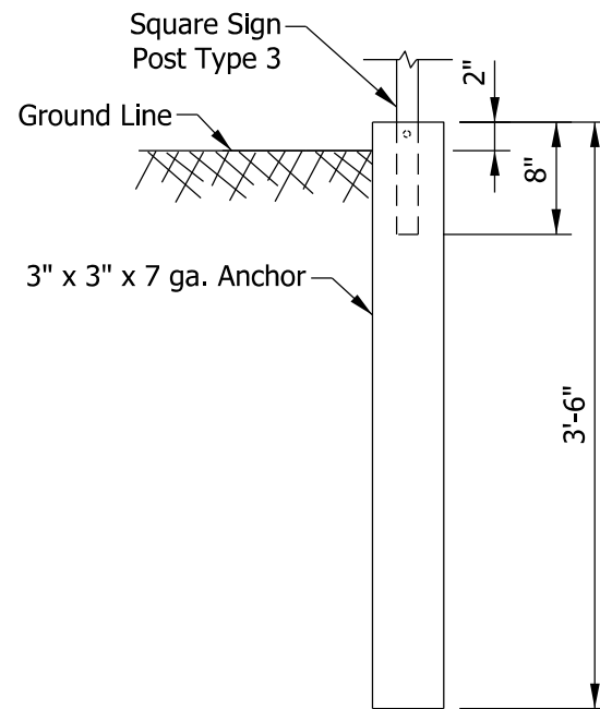
UNREINFORCED ANCHOR BASE
