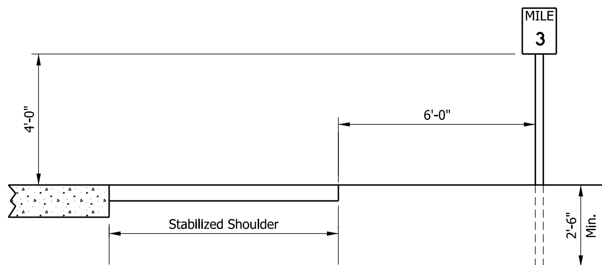
TYPICAL MILE OR REFERENCE POST ①
