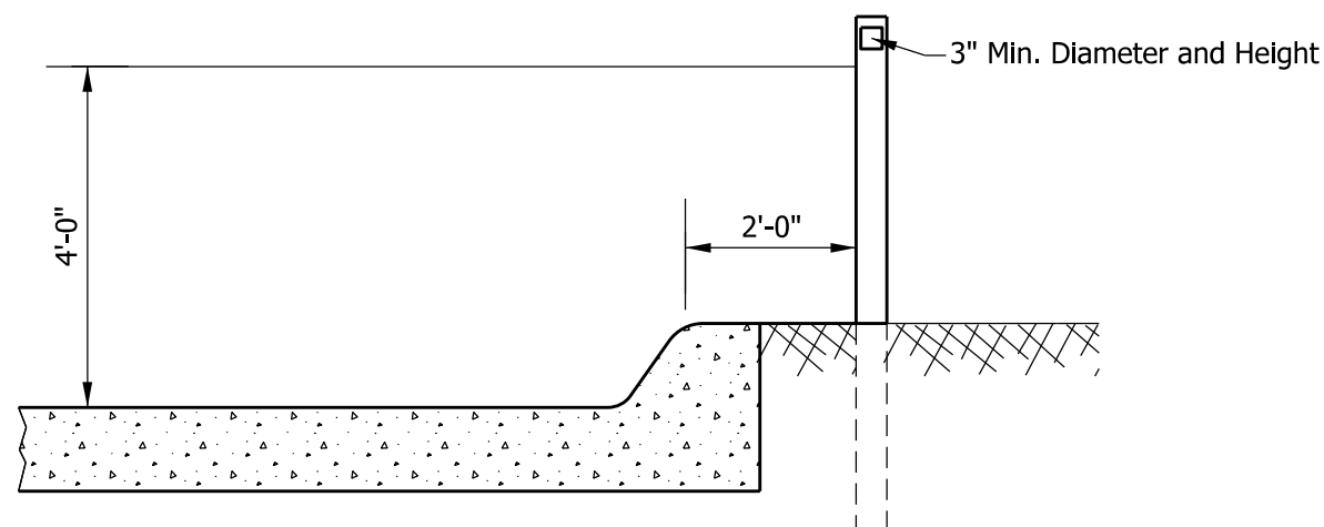
CURB SECTION
