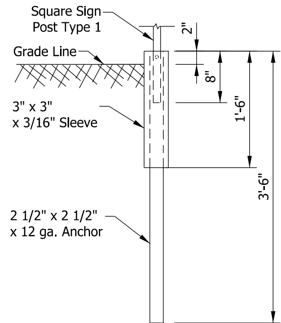
REINFORCED ANCHOR BASE
